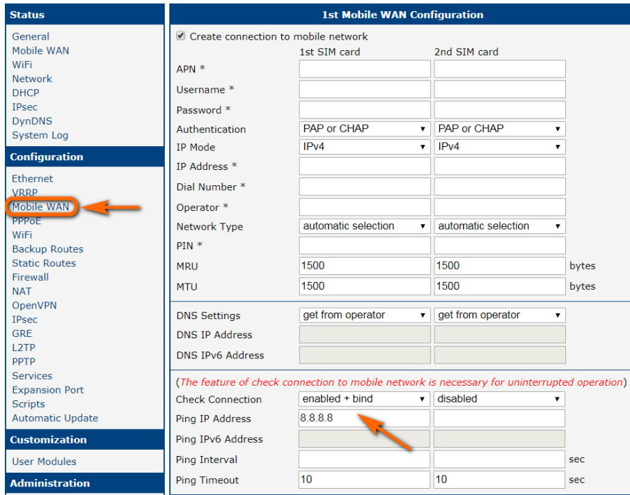
Figure 120: Backup access to the Internet – Mobile WAN configuration
