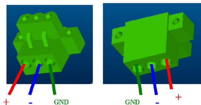
Figure 2.1 Power Connector and Power Lines
