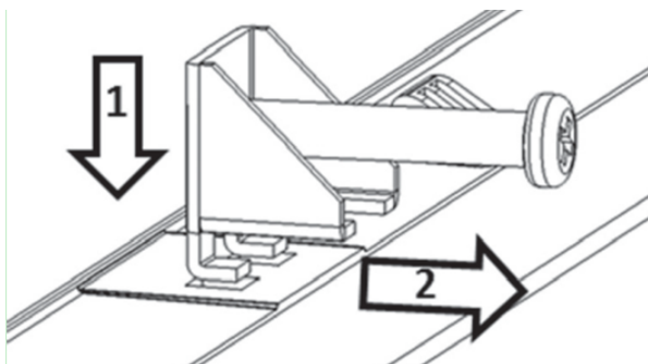
Figure 2.6 Panel Mounting - Clamp Fixing
