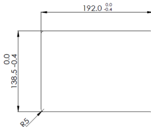
Figure 1.2 Cutout Dimensions
