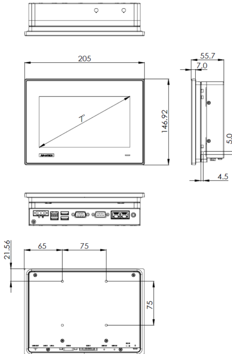
Figure 1.1 Dimensions
