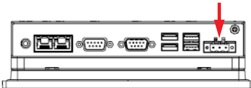
Figure 2.2 Power Connector
