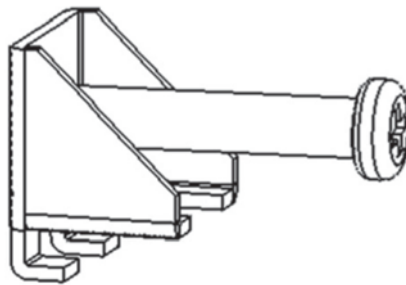
Figure 2.5 Panel Mounting - Clamp with Screw
