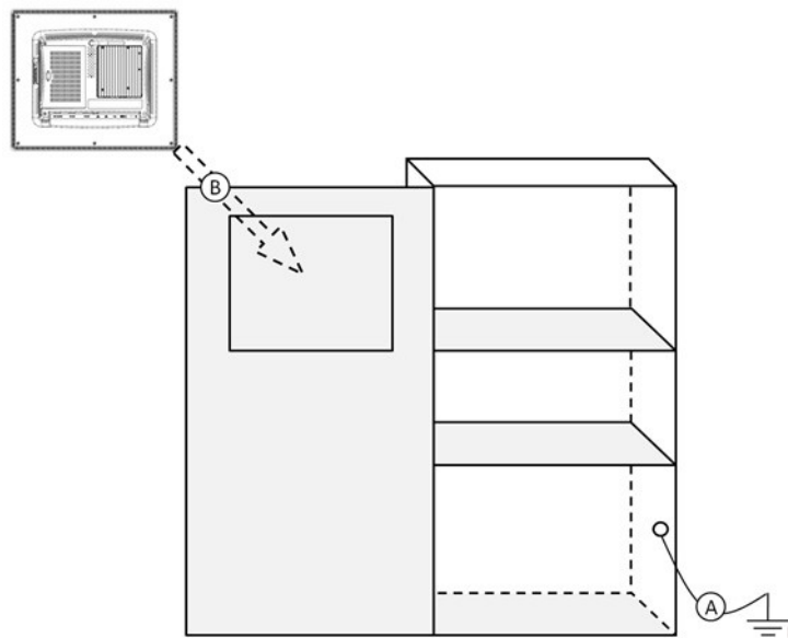
Figure 2.8 Cabinet Installation
