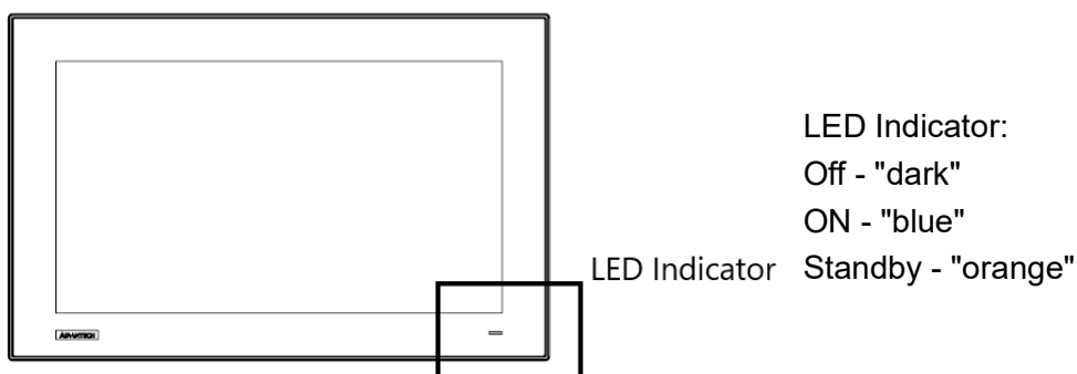
Figure 2.3 Power LED
