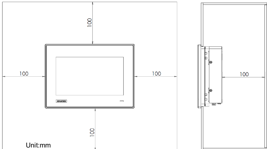
Figure 2.4 Panel Mounting - Positioning
