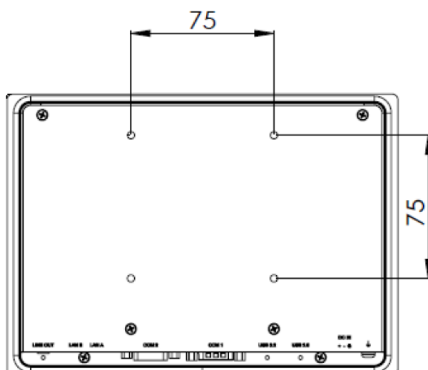
Figure 2.7 VESA Mounting
