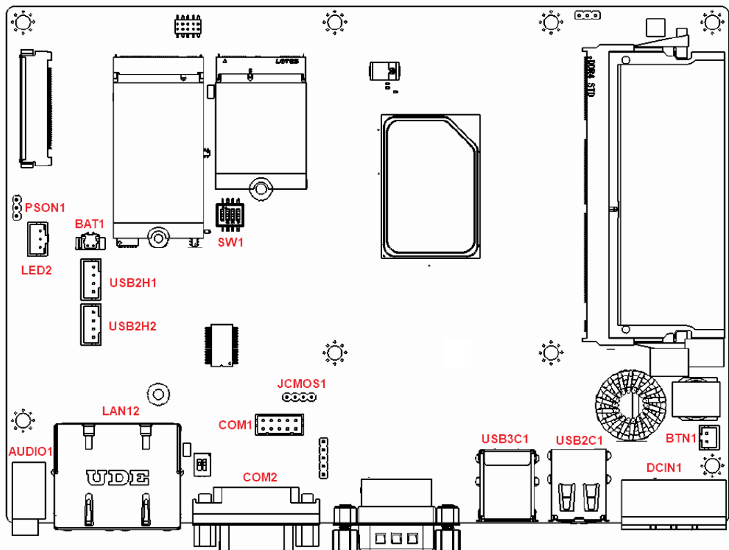
Figure A.1 Board Layout - Top View
