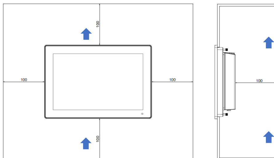
Figure 2.20 Panel Mounting – Positioning
