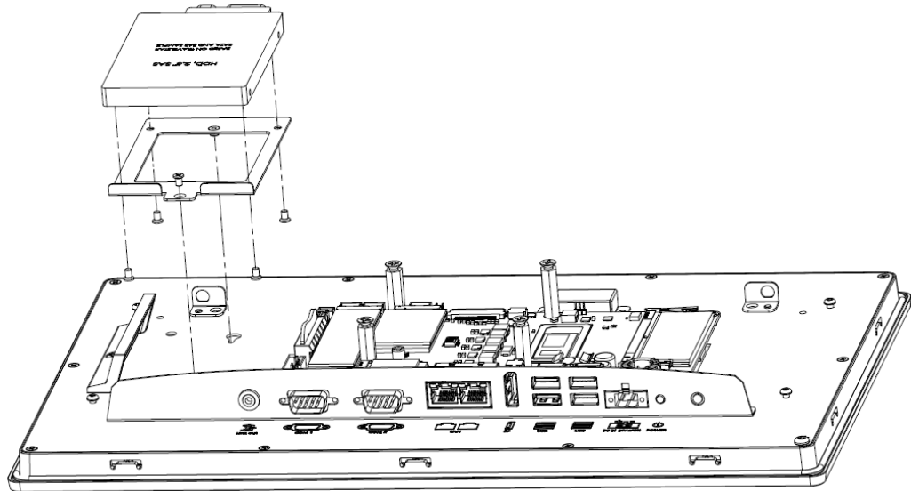
Figure 2.4 SSD Installation
