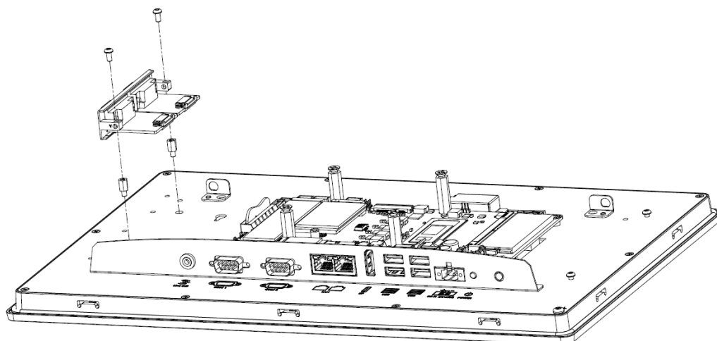
Figure 2.6 iDoor Module Installation
