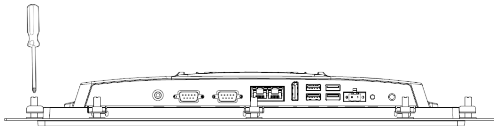
Figure 2.22 Panel Mounting (2)
